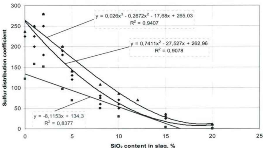
Fig.3 The variation of the sulphur distribution coefficient versus the SiO 2 content in slag
