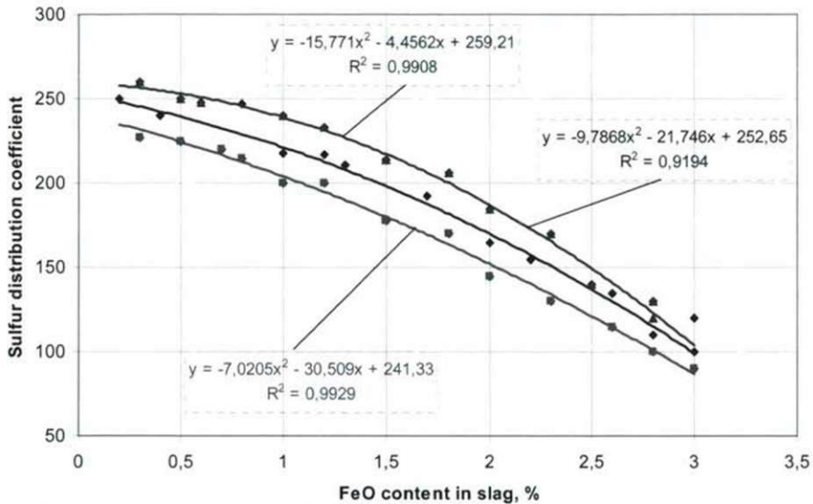
Fig.6 The variation of the sulphur distribution coefficient versus the FeO content in slag
