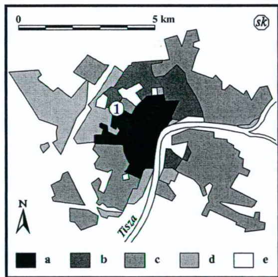
Fig. 1b The built-up types of Szeged [a: centre (2-4-storey buildings); b: housing estates with prefabricated concrete slabs (5-10-storey buildings); c: detached houses (1-2-storey buildings); d: industrial areas; e: green areas, (1): monitoring station]
