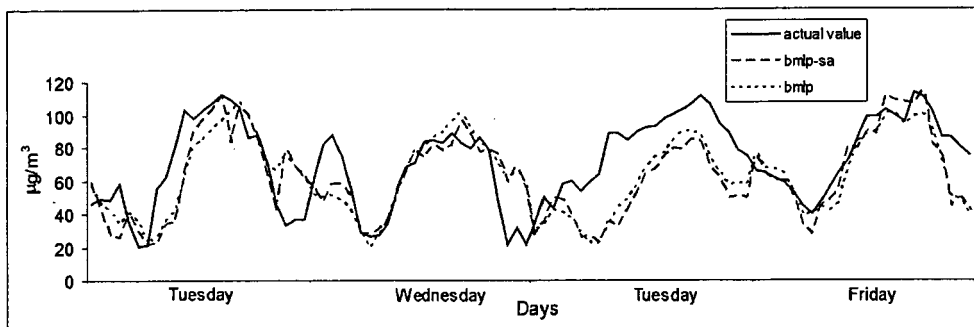
Fig. 4 Estimation of O 3 concentration without external factors
