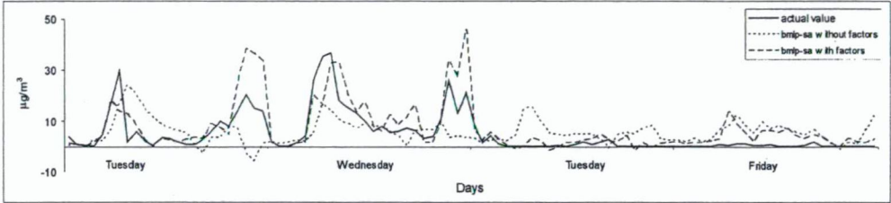
Fig. 6 Estimation of NO concentration using the external factors; NO 2 , O 3 and global radiation
