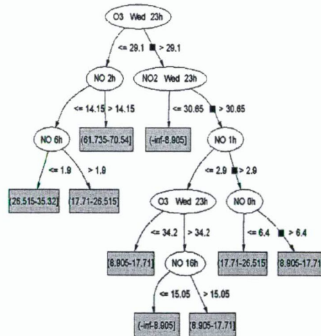
Fig. 9 Part of the decision tree belonging to the estimation of the NO value on Wednesday 23h using the external factors NO 2 , global radiation and O 3 .
