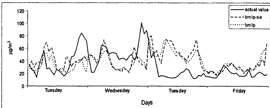
Fig. 3 Estimation of NO_2 concentration without external factors
