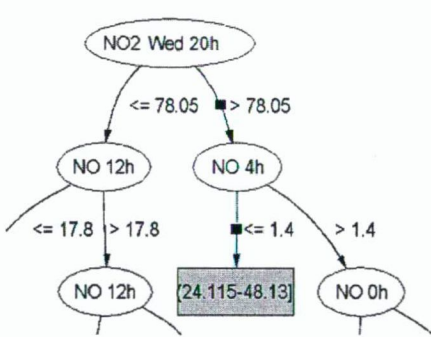
Fig. 7 Estimation of NO 2 concentration using the external factors NO, O 3 and global radiation
