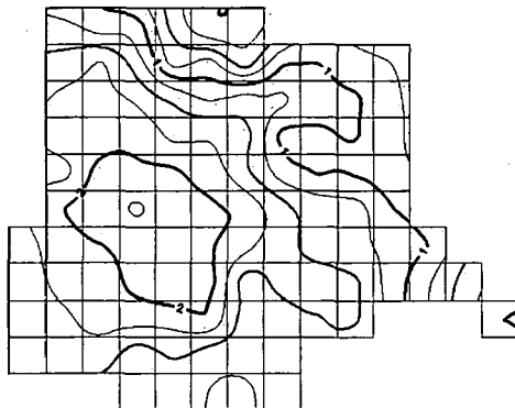
Fig. 3 The spatial structure of the UHI in Debrecen between April 2002 and March 2003. Intensities are in °C. (Szegedi and Kircsi 2003)
