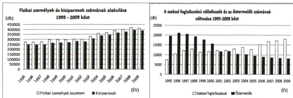
Figure 3. Number of entrepreneurs as physical entities between 1995 and 2009
