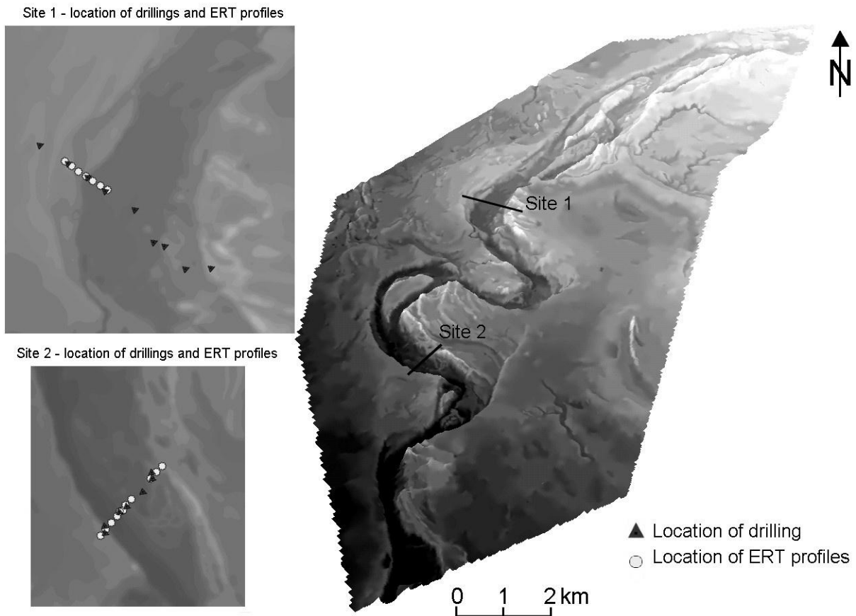
Fig. 2 DEM generated from 1:10000 scale topographic maps with the cross-sections studied in detail
