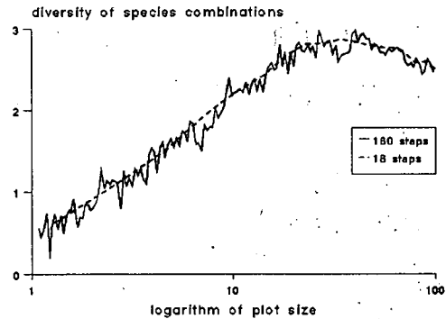
Figure 4. Spatial series analysis of a 4-species community using the diversity of species combinations as a spatial statistics. One of the spatial series curve is produced by large steps while the other is calculated by small steps between the plot sizes. The sample size was 1000 plots for each plot size.
