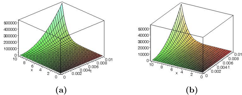
Figure 2: Representing space-fractional solutions of Eq.(26). In (a), solution obtained by the Adomian method for \beta = 1/2 . In (b), solution obtained by the Adomian method for \beta = 1 .
