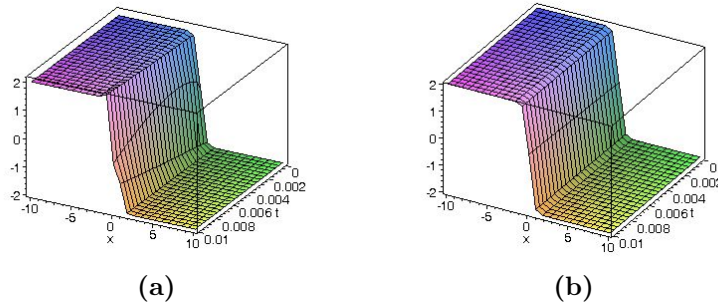
Figure 1: Representing time-fractional solutions of Eq.(20). In (a), solution obtained by the Adomian method. In (b), the exact solution (22).
