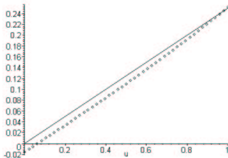
FIGURE 2. The second components of the exact solution (solid line) and its first approximation (drawn with dots)
