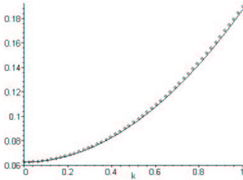
FIGURE 3. The first components of the exact solution (solid line) and its fourth approximation (drawn with dots)
