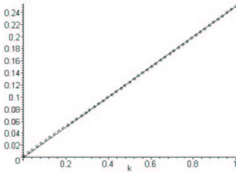
FIGURE 4. The second components of the exact solution (solid line) and its fourth approximation (drawn with dots)
