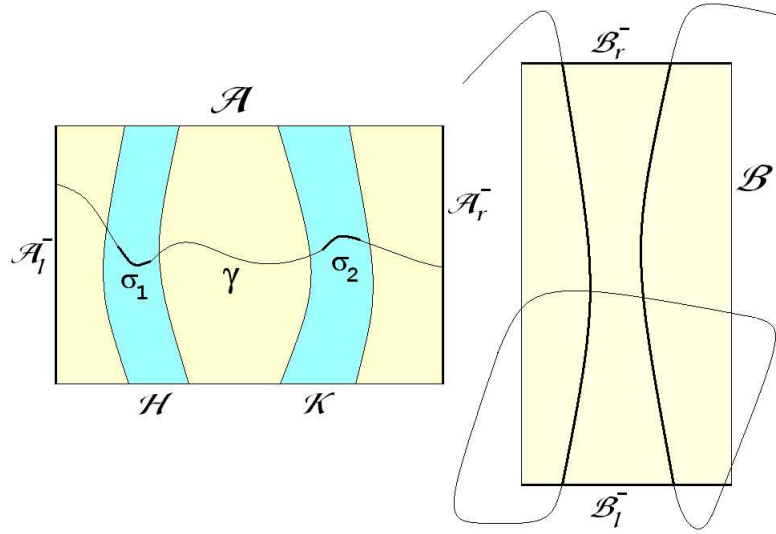
FIGURE 3. A visual explanation concerning Definition 2.1 and Definition 2.2: the rectangles \mathcal{A} and \mathcal{B} , embedded in the plane, have been oriented by selecting, respectively, the sets \mathcal{A}^- and \mathcal{B}^- (drawn by thick lines). We have darkened two compact subsets \mathcal{H} and \mathcal{K} of \mathcal{A} . In the picture, we describe the action of a map \phi such that (\mathcal{H}, \phi) : \tilde{\mathcal{A}} \rightleftarrows \tilde{\mathcal{B}} and also (\mathcal{K}, \phi) : \tilde{\mathcal{A}} \rightleftarrows \tilde{\mathcal{B}} . For a path \gamma : [0, 1] \rightarrow \mathcal{A} with \gamma(0) and \gamma(1) belonging to different components of \mathcal{A}^- , we have put in evidence two restrictions (sub-paths) \sigma_1 and \sigma_2 with range in \mathcal{H} and \mathcal{K} , respectively, such that their composition with \phi determines two new paths (drawn by bolder vertical lines) with values in \mathcal{B} and connecting the two different components of \mathcal{B}^- . In this case, we could also write \phi : \tilde{\mathcal{A}} \rightleftarrows^2 \tilde{\mathcal{B}} .
