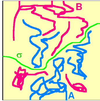
FIGURE 2. A pictorial explanation to the proof of Lemma 2.1.
