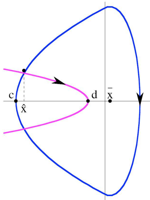
FIGURE 11. Example of a trajectory of (E_r) (drawn with a darker line) overlapped with a trajectory of (E_s) . The times for moving a point along an orbit from c to \hat{x} or from \hat{x} to d can be explicitly determined by means of time-mappings integrals.
