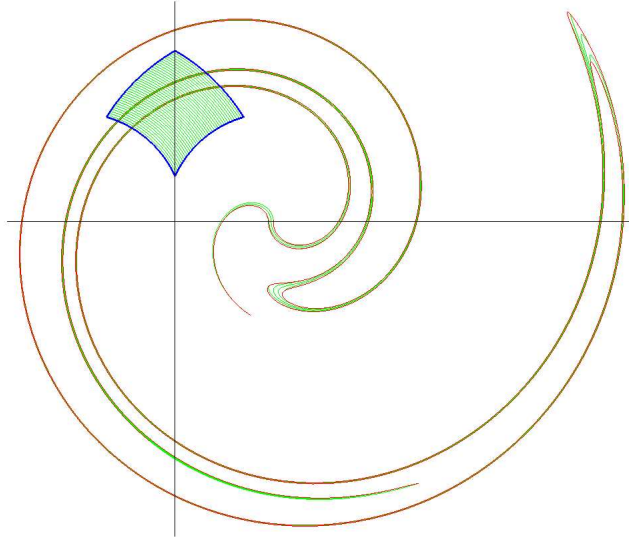
FIGURE 5. For r, p_1, p_2, q_1, q_2 and f_1 as in Fig. 4, we have also fixed the parameters of f_2 by taking a_2 = 0.9 and e_2 = 0 . The present picture shows the image of \mathcal{P} through the composite map f_2 \circ f_1 . It is evident that (f_2 \circ f_1)(\mathcal{P}) crosses \mathcal{P} twice in the correct way.
