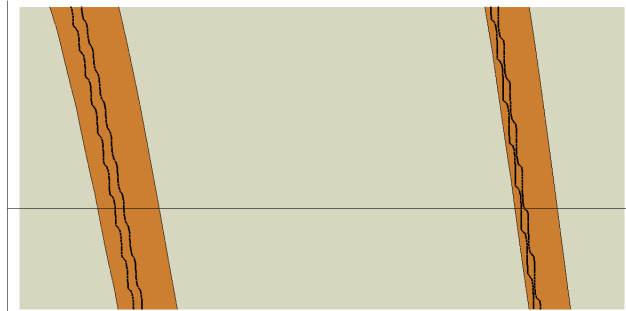
FIGURE 9. In the simple case of Example 3.2 and for f_1 and f_2 determined by the coefficients chosen for drawing Fig. 8, we can determine the sets \mathcal{H}_1 and \mathcal{H}_2 in Theorem 3.1. Indeed, in the set \mathcal{P} , transformed in the rectangle [p_1, p_2] \times [q_1, q_2] by a suitable change of coordinate, we have found two subsets (drawn with a darker color) whose image through f_1 are contained in \mathcal{O} . Inside these subsets, we have found two smaller domains such that their images through f_2 \circ f_1 are contained again in \mathcal{P} . Clearly, any path contained in the rectangle [p_1, p_2] \times [q_1, q_2] and joining the left to the right sides contains two sub-paths which are stretched by the composite mapping to paths connecting again the left and the right sides. Up to a homeomorphism between \mathcal{P} and [p_1, p_2] \times [q_1, q_2] , this is precisely what happens in (\mathcal{P}, \mathcal{P}^-) for f_2 \circ f_1 .
