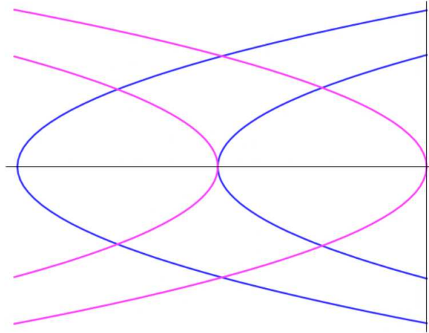
FIGURE 12. Level lines of system (E_r) overlapped with the level lines of system (E_s) in the left half plane x \leq 0 . The sets \mathcal{P} and \mathcal{O} are those bounded by the four different level lines and contained in the lower half plane y \leq 0 and in the upper half plane y \geq 0 , respectively.
