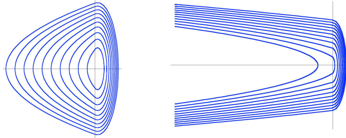
FIGURE 10. Trajectories of system (E_r) (left) and system (E_s) (right). For this example we have chosen k = 10 , r = 4 and s = 0.5 .
