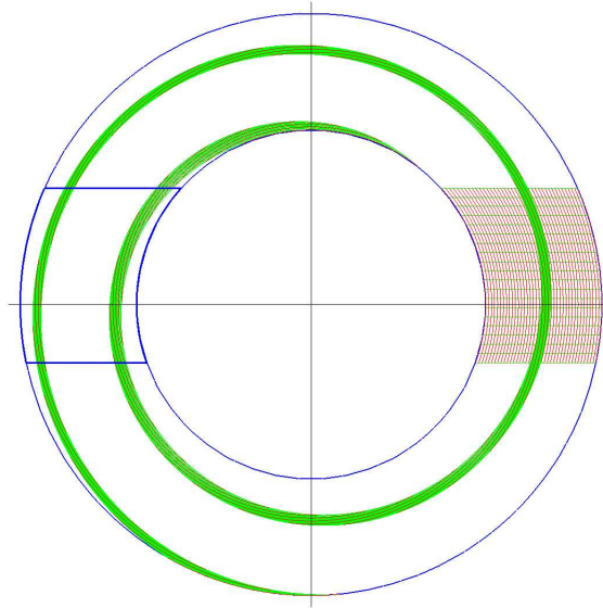
FIGURE 6. A pictorial comment to condition (H_f) of Theorem 3.1, with reference to Example 3.2. We have chosen p_1 = 3 , p_2 = 5 , q_1 = -1 and q_2 = 2 in order to determine the annulus A[p_1, p_2] centered at the origin and the strip S[q_1, q_2] which goes across it. For the map f_1 we have taken e_1 = 0.4\pi and c_1 = 3\pi . We define the set \mathcal{P} of Theorem 3.1 as the right hand side intersection of the annulus with the strip and select the two components of \mathcal{P}^- as the intersections of \mathcal{P} with the inner and outer boundaries of the annulus. The set \mathcal{O} is defined as the left hand side intersection of the annulus with the strip and the two components of \mathcal{O}^- are the intersections of \mathcal{O} with the lower and upper sides of the strip. The narrow band, spiralling inside the annulus, is the image of \mathcal{P} under f_1 . Clearly, any path in \mathcal{P} joining the two components of \mathcal{P}^- is transformed by f_1 onto a path crossing \mathcal{O} twice in the correct manner.
