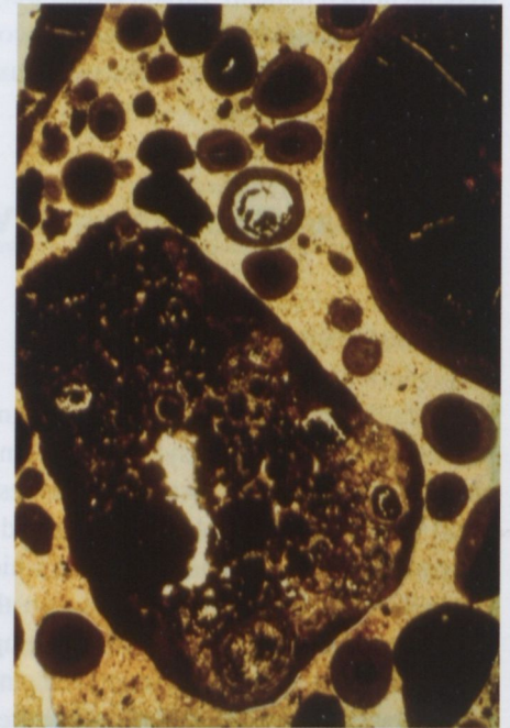
Fig. 7. Thin section photomicrograph of gravelly bauxite from the Bagolyhegy deposit (width of the photo is ~1 mm).
