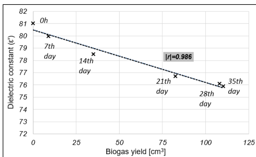
Figure 3. The connection between the dielectric constant and bigos yield during the anaerobic co-digestion process
