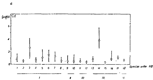
d) Cd
