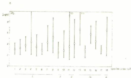
c) Pb
